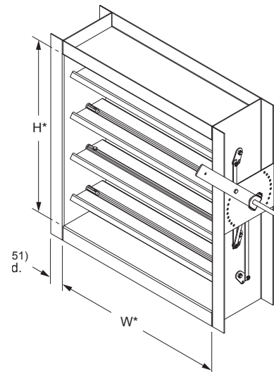
Model AC-82 *Damper dimensions furnished approximately net I.D..
