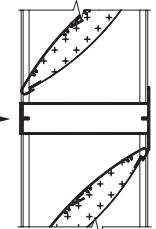
Horizontal Mullion (standard)
