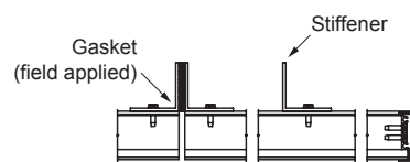
Hidden Vertical Mullion (optional)
