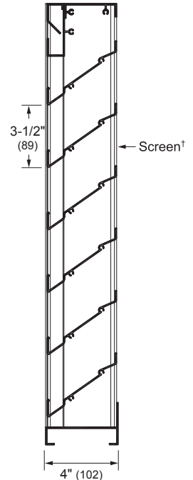
Vertical Section
