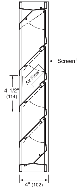
Vertical Section
