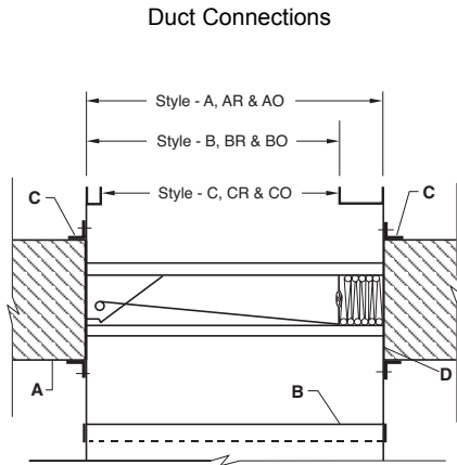
Damper Installation ( 2-sided Mounting Angle )
