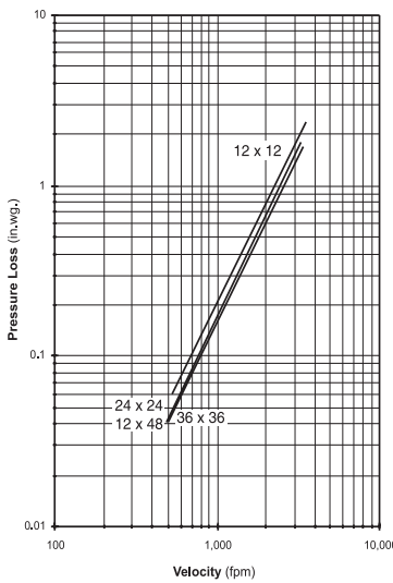
Figure 5.5 Plenum Mount
