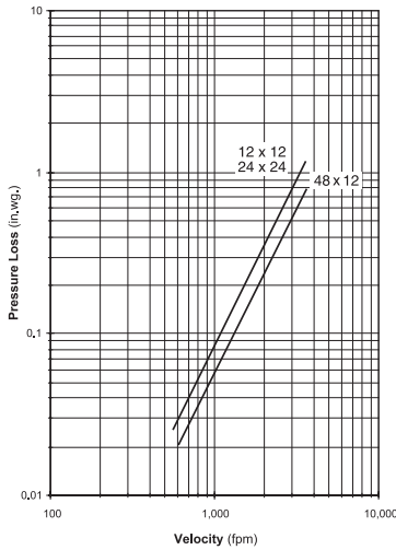
Figure 5.2 — Ducted Inlet
