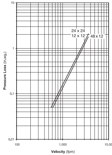
Figure 5.5 Plenum Mount
