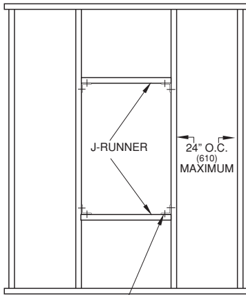
Opening Preparation Detail
