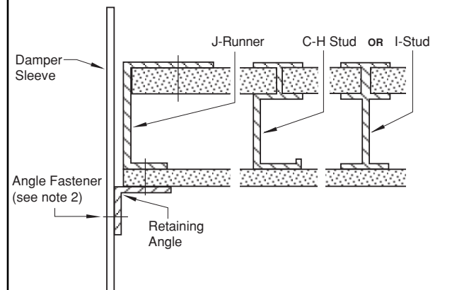
Wall with Single Layer of Drywall
