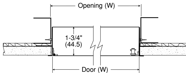
Model PW Typical Wall Installation
