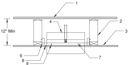
Damper with Extended Sleeve
