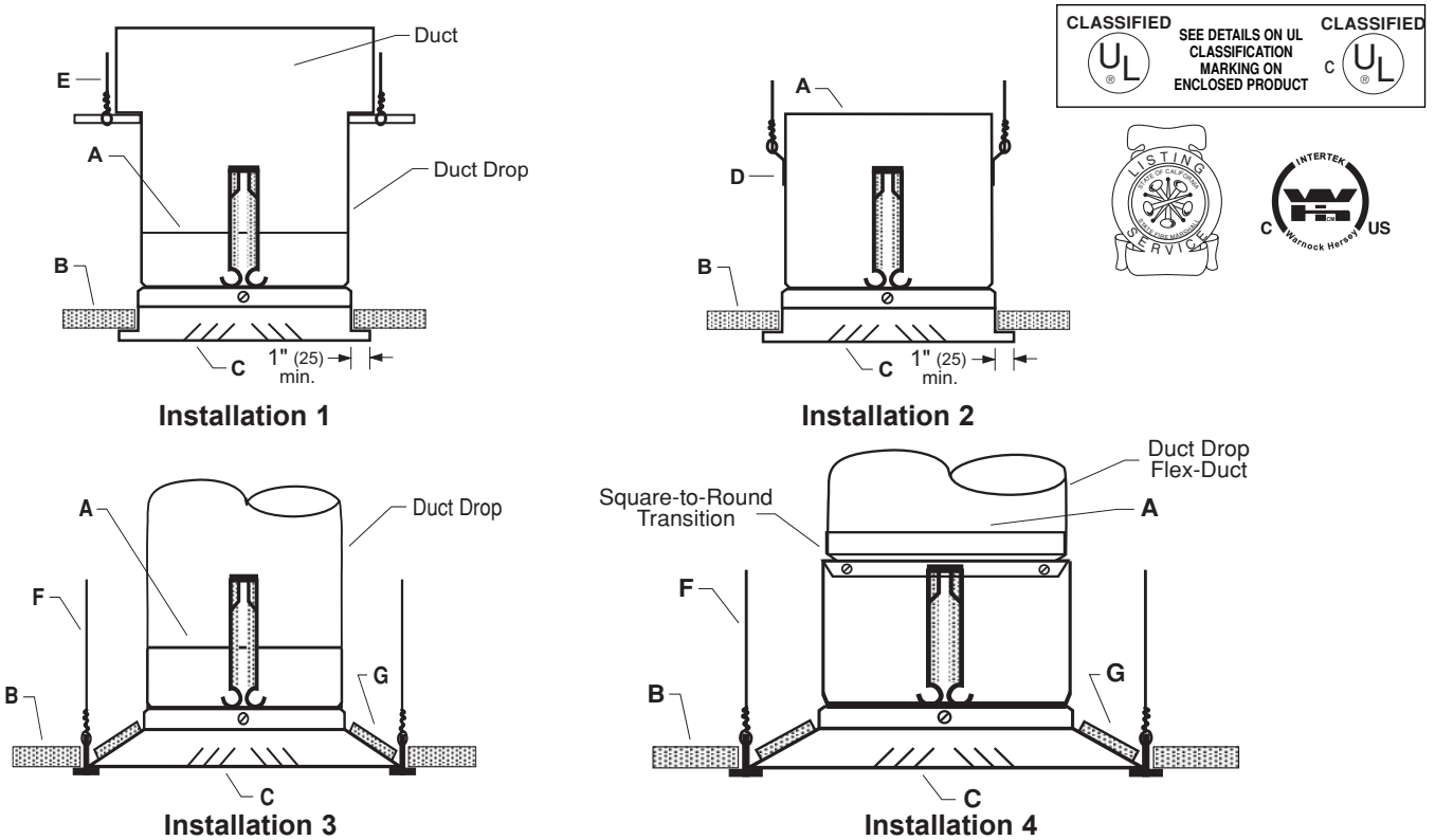
Illustrations show RD2 type damper, model RD8 similar.
