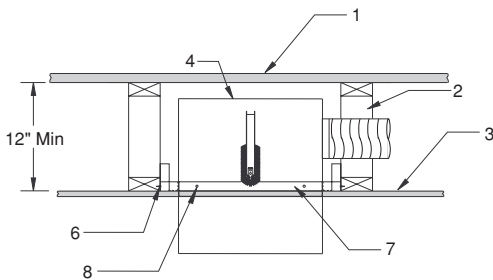
Damper with Extended Sleeve
