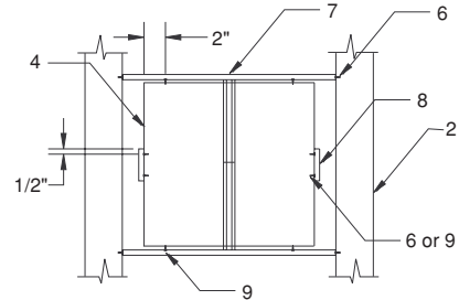
Top View of Damper
