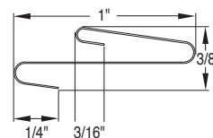
Standard Boot Rail
