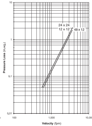
Figure 5.5 Plenum Mount
