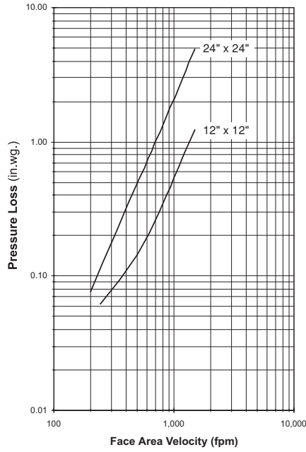
Figure 5.5 — Plenum Mount
