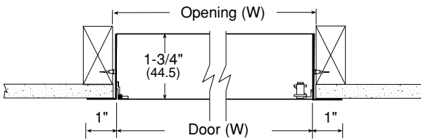
Model WB Typical Wall Installation
