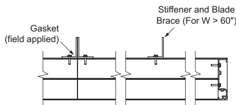
Hidden Vertical Mullion (optional)
